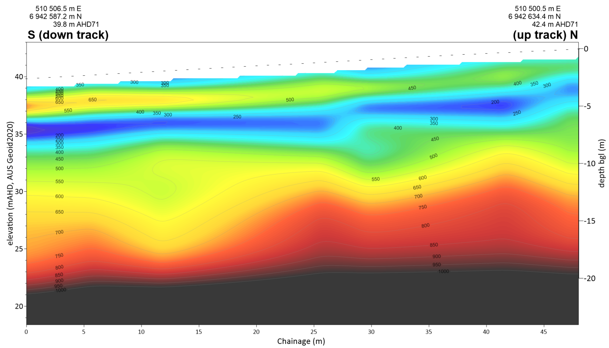
Seismic Line MASW AU-GP 130
